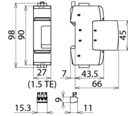
Dimension drawing DG SE DC 242 FM
